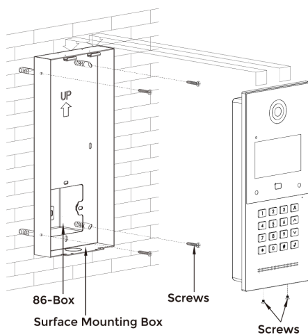
Surface mounting — 86 mounting box
