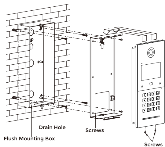
Flush mounting
